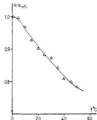
Figure 4. Temperature dependence of the quantum yields of chemiluminescence of 1d (4-(dimethylamino)phthalhydrazide) and of fluorescence (4-(dimethylamino)phthalate, 2d ): \Delta , chemiluminescence; full line, fluorescence. The fluorescence was measured in a pH 12 solution containing 5 \times 10^{-5} M phthalate 2d . The excitation wavelength was 255 nm. The chemiluminescence yield was measured upon pulsed e^- -beam irradiation of an O_2 -saturated solution containing 0.1 M N_3^- , 10^{-3} M hydrazide 1d holding pH 14.
