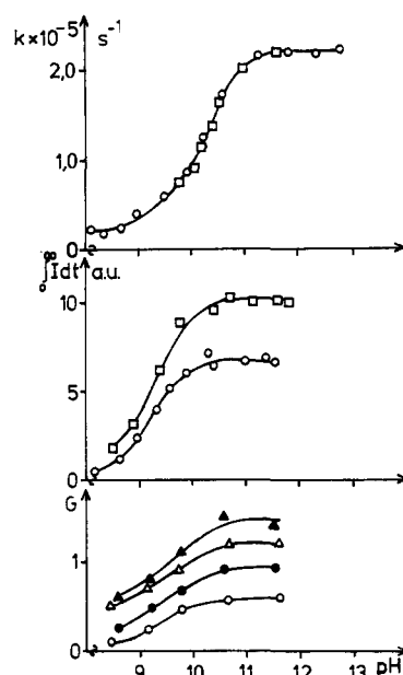
Figure 1. (Top) pH dependence of the rate constant for hydroperoxide decomposition as extracted from the build up of e^- -beam initiated chemiluminescence: \circ , 10^{-3} M luminol ( 1b ), O_2 saturated (reaction 2); \square , 10^{-2} M luminol, H_2O_2 varied from 0.03 M at pH > 11 to 0.1 M at pH 9.8, N_2O saturated (reaction 3). (Middle) pH dependence of the total chemiluminescence yield: \circ , 10^{-3} M luminol, O_2 saturated (reaction 2); \square , 10^{-3} M luminol, 10^{-2} M H_2O_2 , N_2O saturated (reaction 3). (Bottom) variation of radiolytic G values with pH as found in e^- -beam irradiated solutions: \circ , G(3\text{-aminophthalate}) ( 2b ), 10^{-3} M luminol, O_2 -saturated solutions (reaction 2); \bullet , G(-\text{luminol}) , same as above; \blacktriangle , G(3\text{-aminophthalate}) , 10^{-3} M luminol, 10^{-2} M H_2O_2 , N_2O -saturated solutions (reaction 3); \blacktriangle , G(-\text{luminol}) , same as above. All experiments were carried out at 20^\circ \text{C} in solutions containing 1 M CO_3^{2-} throughout.
