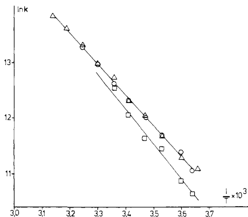
Figure 3. Arrhenius plots for the decomposition of the hydroperoxide 5 generated from ( \square ) 1c (4-aminophthalhydrazide) at pH 12.4, ( \circ ) 1b (luminol) at pH 12.4, ( \Delta ) 1d (4-(dimethylamino)phthalhydrazide) at pH 14.0. All solutions were saturated with O_2 and contained 10^{-3} M hydrazide and 0.1 M N_3^- .
