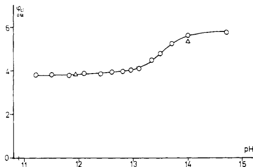
Figure 5. pH dependence of the chemiluminescence quantum yield of 1d (4-(dimethylamino)phthalhydrazide): O, pulse radiolytically determined light yield in O_2 -saturated solutions containing 10^{-3} M hydrazide and 0.1 M N_3^- ; \Delta , light yield obtained in the reaction between the hydrazide 1d and H_2O_2 with hemine as the catalyst (ref 39). The values are relative and normalized to the one obtained at pH 12.
