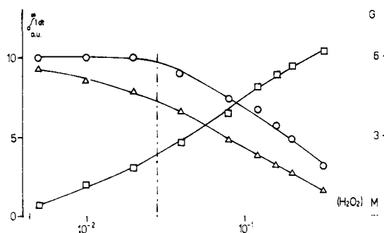
Figure 2. The total pulse radiolytical yields of chemiluminescence and of radicals formed initially as functions of H 2 O 2 concentration (conditions: pH 10.6, 10 -3 M luminol ( 1b ), 0.5 M CO 3 2- , N 2 O saturation): ○, total experimental light yield; △, measured initial yield of diazasemiquinone radicals 4b ; □, initial yield of O 2 •- ; full line, through circles; light yield calculated by use of the initial radical yields and the measured ratio 2k 1 /k 2 = 2.2 and assuming equal chemiluminescence efficiencies in reactions 2 and 3; broken line, H 2 O 2 concentration at which reactions 2 and 3 have equal weights.
